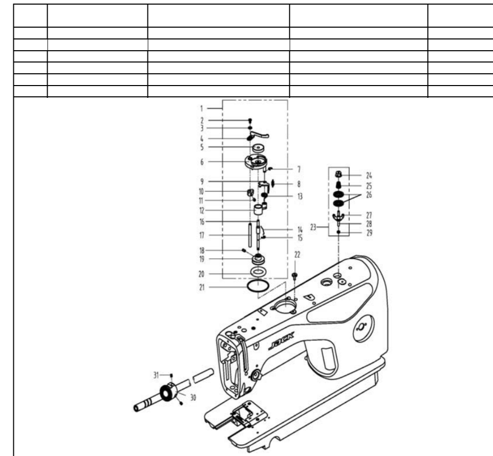
12. /Oil Ceservoir,Knee Lifter Components
